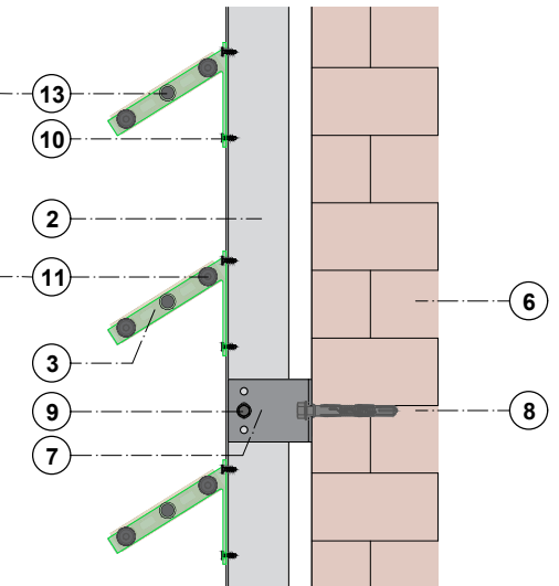
VERTICAL SECTION SCALE: 1/8
